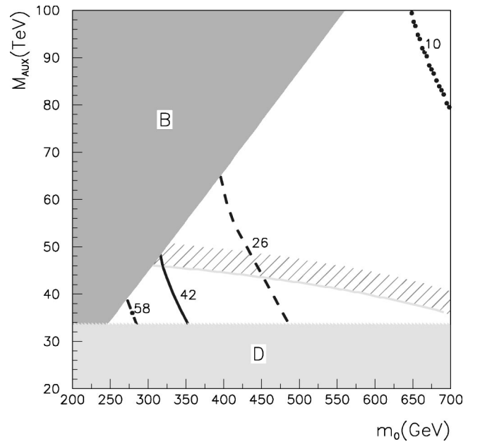
FIG. 13. Contour plot on the plane of (m_0, M_{\text{aux}}) in the minimal anomaly-mediated model with \tan\beta = 30 .
